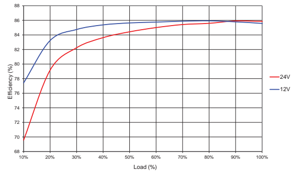
NCS12S4805C
