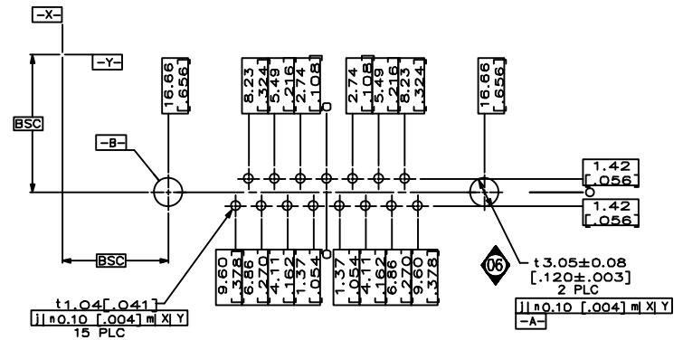
P.C. BOARD MOUNTING DIMENSIONS
