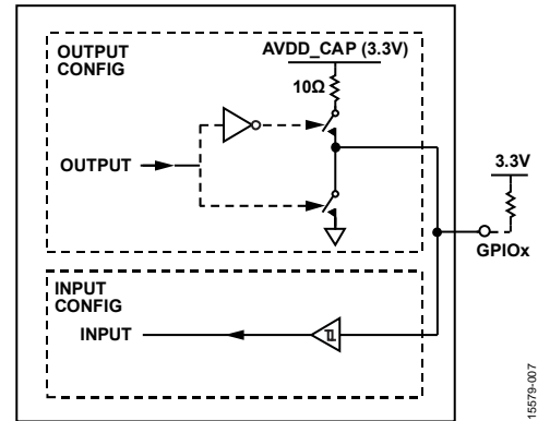
Figure 11. GPIOs
