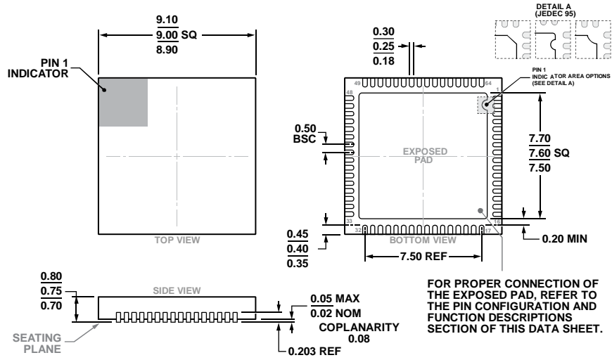
Figure 30. 64-Lead Lead Frame Chip Scale Package [LFCSP] 9 mm × 9 mm Body and 0.75 mm Package Height (CP-64-15) Dimensions shown in millimeters
