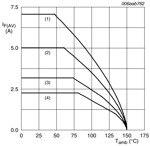
Ceramic PCB, Al_2O_3 , standard footprint T_j = 150\text{ }^{\circ}C (1) \delta = 1 ; DC (2) \delta = 0.5 ; f = 20\text{ kHz} (3) \delta = 0.2 ; f = 20\text{ kHz} (4) \delta = 0.1 ; f = 20\text{ kHz}
