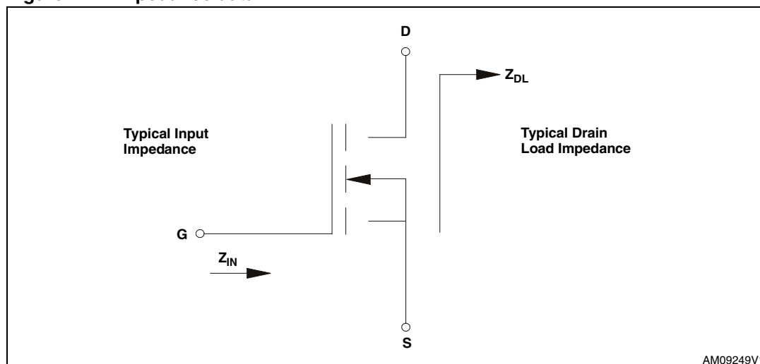
Figure 2. Impedance data
