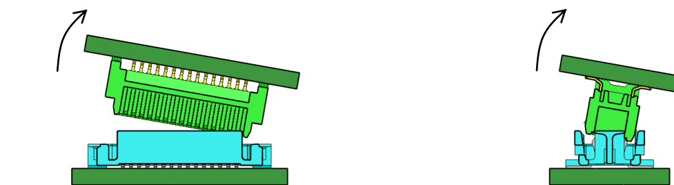
図-5 こじり抜去 Figure-5 Withdrawal with twisting the connector at an angle
