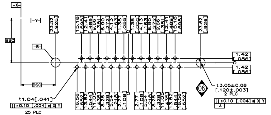
P.C. BOARD MOUNTING DIMENSIONS
