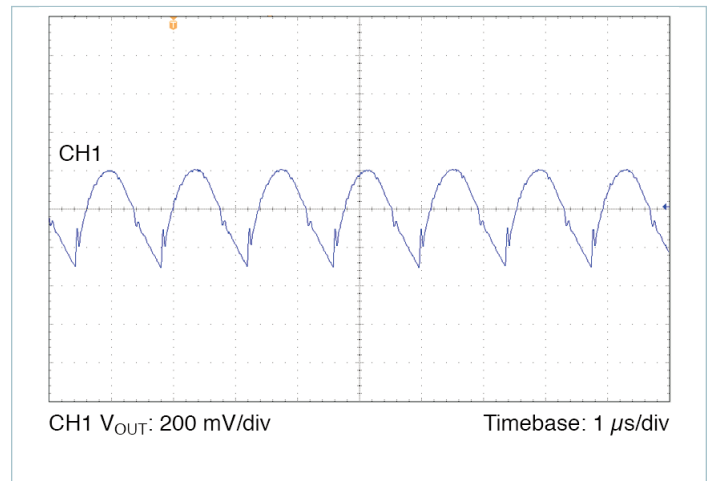
Figure 19 — Output voltage ripple, V_{IN} = 270\text{ V} , V_{OUT} = 12.0\text{ V} , C_{OUT\_EXT} = 1000\text{ }\mu\text{F} , R_{LOAD} = 0.100\text{ }\Omega
