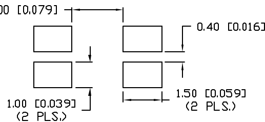
RECOMMENDED SOLDER PAD LAYOUT
