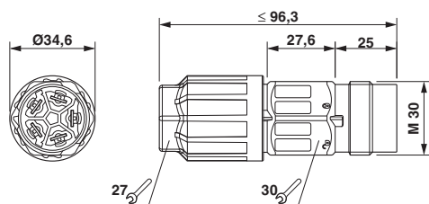
QPD C 5x2.5 dimensional drawing
